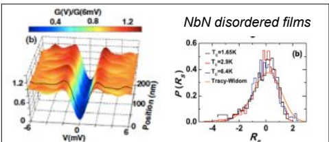
The inhomogeneous local DOS measured by STM shows an universal probability distribution of the local SC order parameter when properly rescaled
