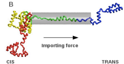
Fig. Transport of a protein by a pulling force
