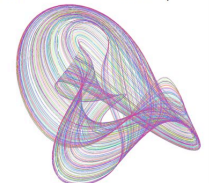
Fig. A strange attractor showing a fractal structure.
