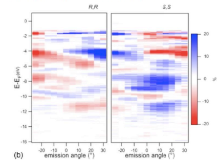
Maps of the dichroic signal for two enantiomers of chiral molecules, acquired by angular resolved photoemission with circularly polarized light Ferrari L. e al. Phys.Rev. B 91, 085408 (2015)
